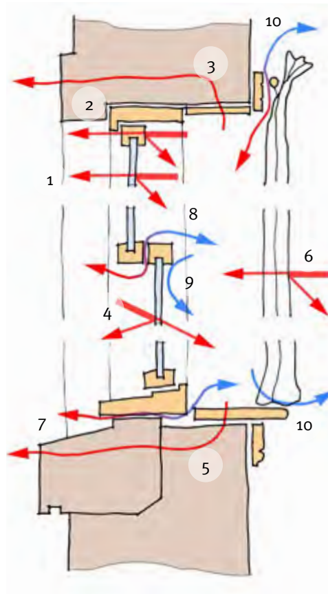
Diagram showing the 10 ways in which buildings can gain and lose heat through windows
