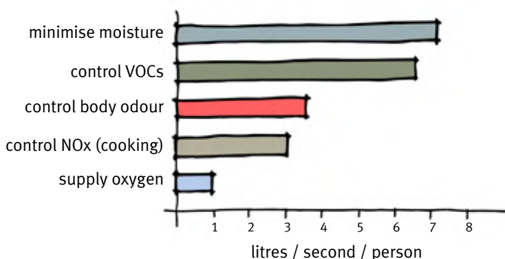
Graph showing ‘pollution sources’ in a typical home and their relative impact on the ventilation rates required by the building standards (in England and Wales)
