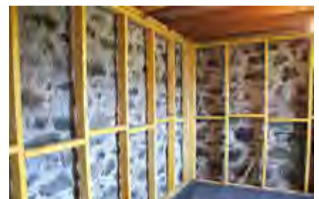
Installing an internal frame, infilled with insulation and a plasterboard finish is relatively simple and inexpensive. In this example, the frame is set apart from the wall to avoid moisture in the stonework affecting the new works.
