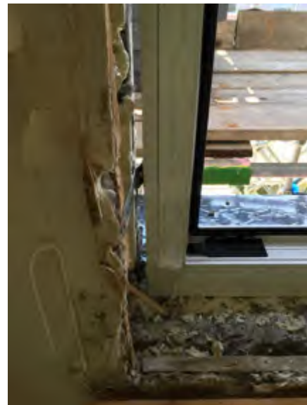
Brand new windows installed but note the gap around the frame which is normally sealed with expanding foam
